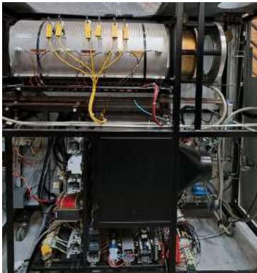
Refurbishment of a multi-process tubular furnace
